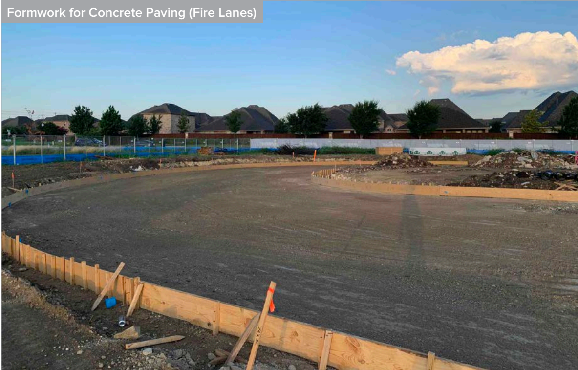
Reinforcing and Formwork for Concrete Paving (Fire Lanes)
